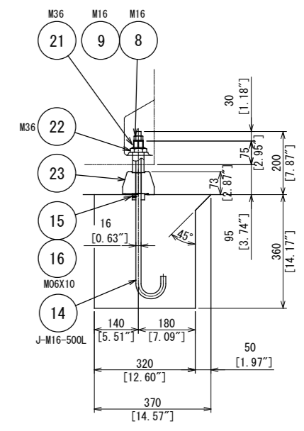
C DETAIL (S=1:6) (6 PLACES)
